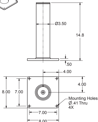
Pedestal base
