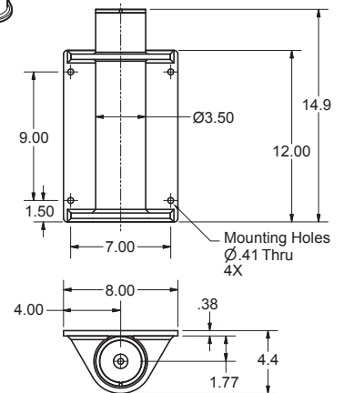
Wall-mounted base
